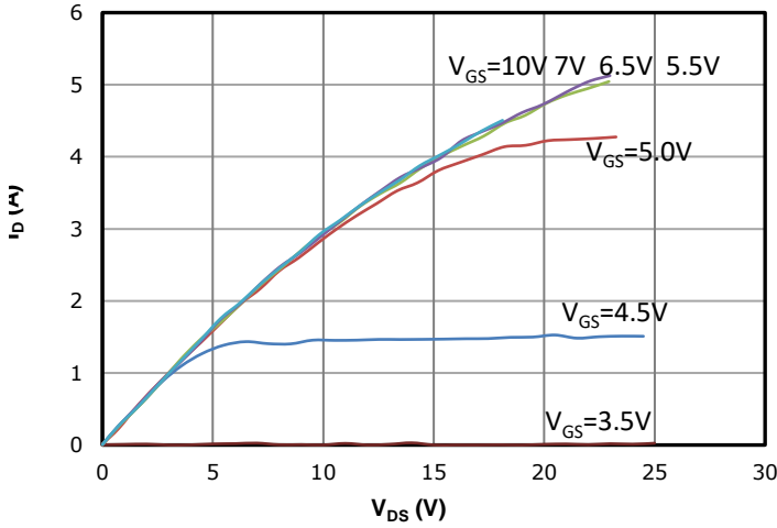
Fig 1: Output Characteristics
