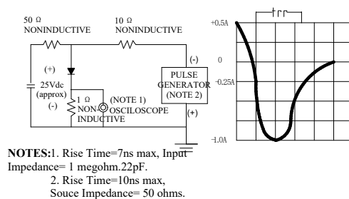
FIG.6-TEST CIRCUIT DIAGRAM AND REVERSE RECOVERY TIME CHARACTERISTIC
