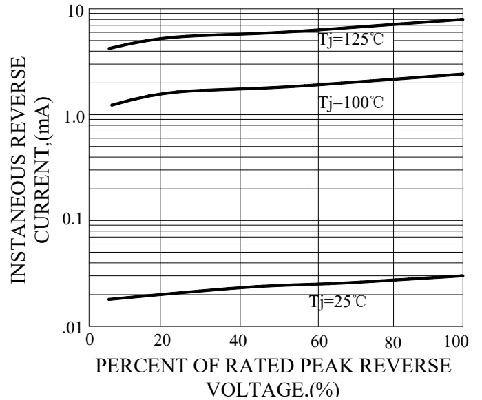
FIG.4-TYPICAL REVERSE CHARACTERISTICS
