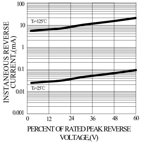
FIG.4-TYPICAL REVERSE CHARACTERISTICS
