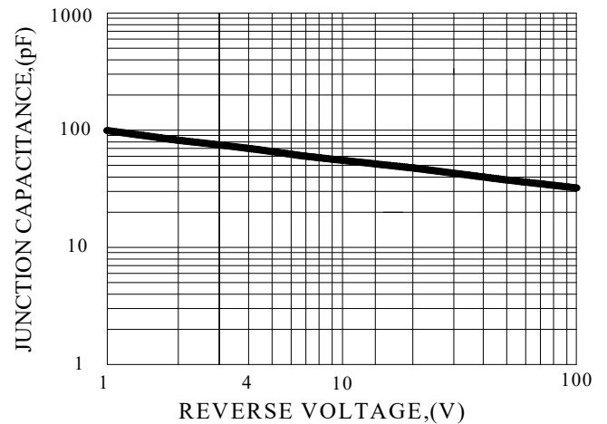
FIG.4-TYPICAL JUNCTION CAPACITANCE
