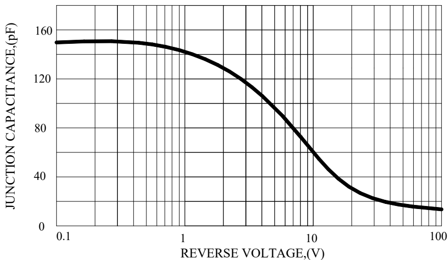
FIG.5-TYPICAL JUNCTION CAPAOTANCE
